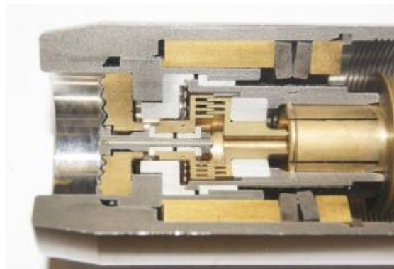
FIGURE 10.32: Cutaway view of a diaphragm pressure sensor with capacitive sensing—diaphragm on the left, electrodes of capacitive sensor in the middle—photo author
