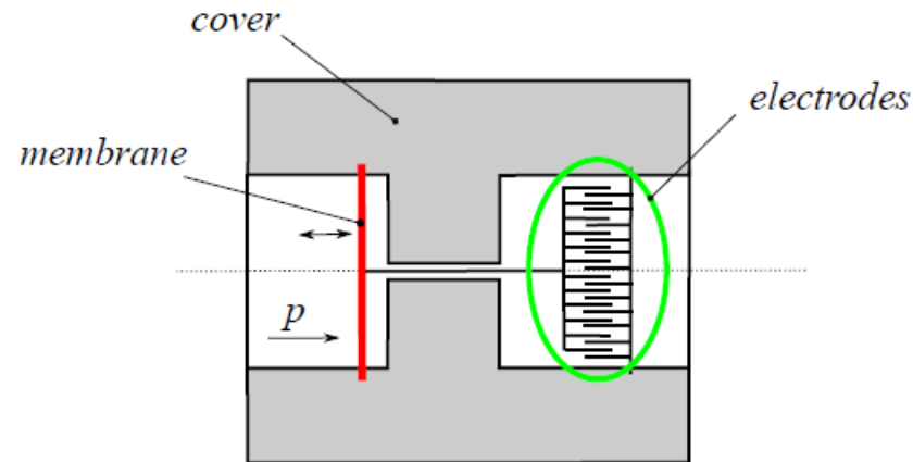
FIGURE 10.31: Principle of diaphragm pressure sensor with capacitive sensing
