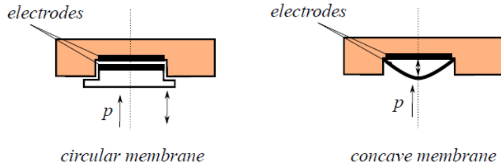
FIGURE 10.28: Principle of diaphragm pressure sensor with capacitive sensing
