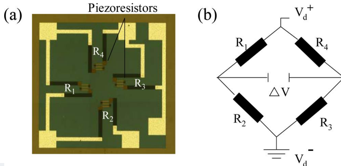
FIGURE 10.23: Principle of diaphragm sensor with piezoresistors
