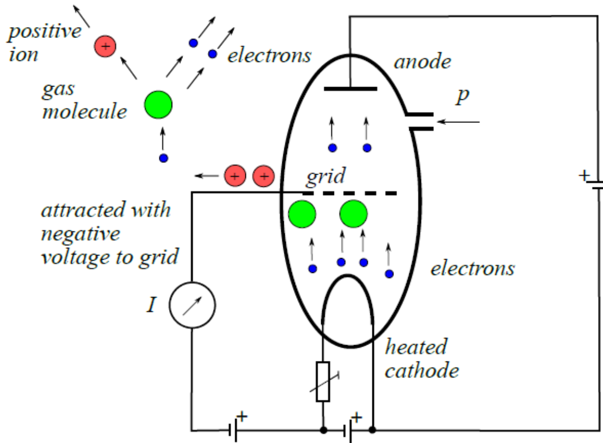
FIGURE 10.42: Ionization pressure sensor
