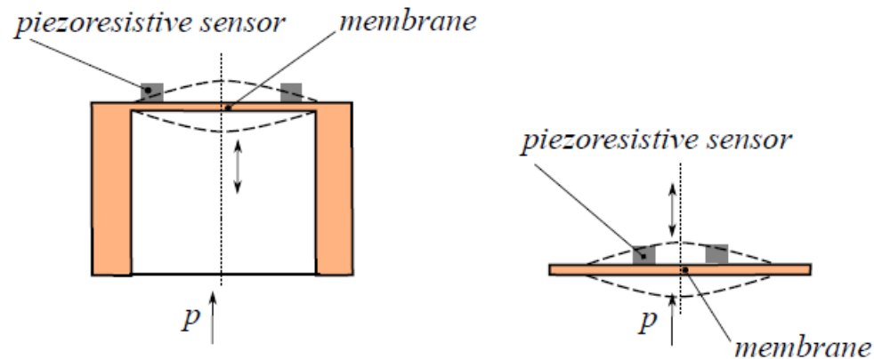
FIGURE 10.23: Principle of diaphragm sensor with piezoresistors
